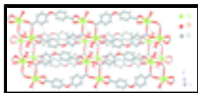
Fig. 3. View of three-dimensional supramolecular structure with hydrogen bond interactions shown as dashed lines.
