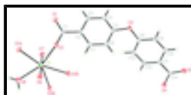
Fig. 1. Thermal ellipsoid plot of a portion of the title compound, showing the atom-labelling scheme. Displacement ellipsoids are drawn at the 30% probability level [symmetry codes (A): -x + 1, -y + 1, -z + 1 ; (B): -x + 2, -y + 1, -z + 1 ].
